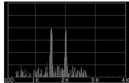
SPECTRUM DISPLAY
