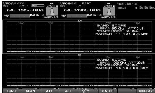
"SPECTRUM SCOPE" Screen
