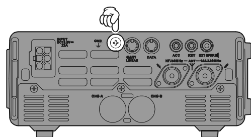
GND Terminal
