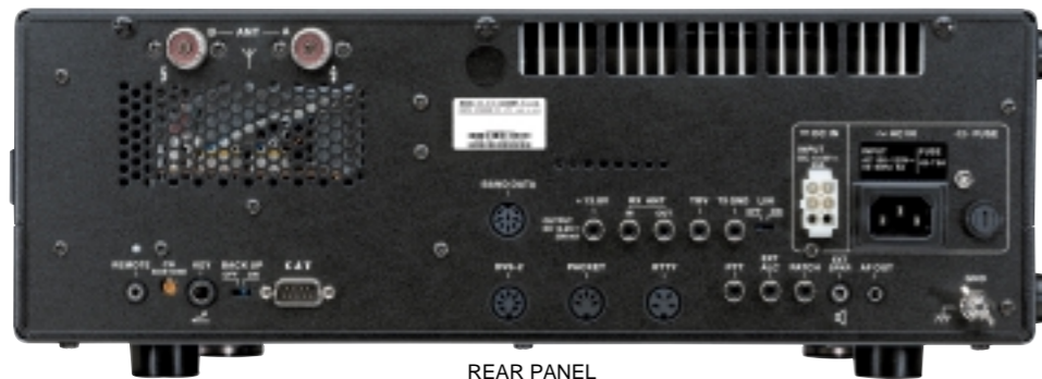
REAR PANEL
