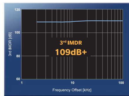
14MHz Band 3rd Intermodulation Dynamic Range (IMDR)
