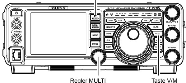
Taste F(M-LIST)
